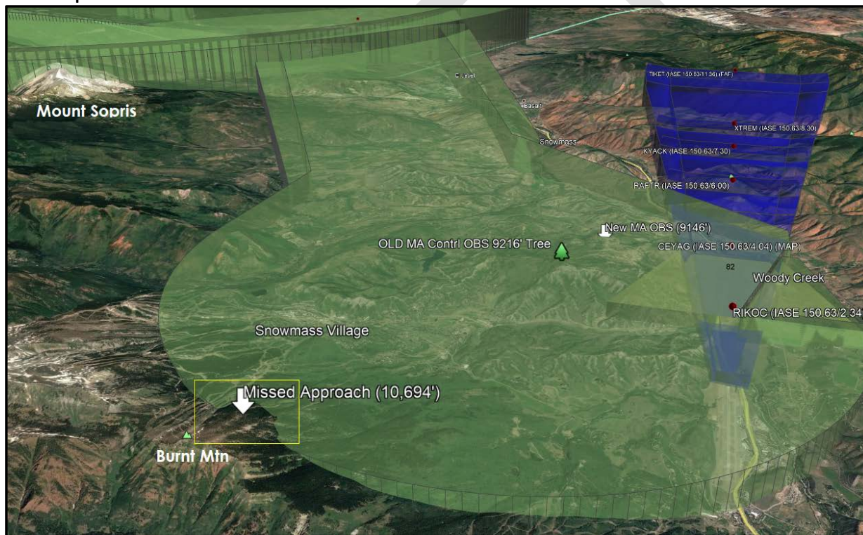
Aerial Depiction of M.A. Obstacles
