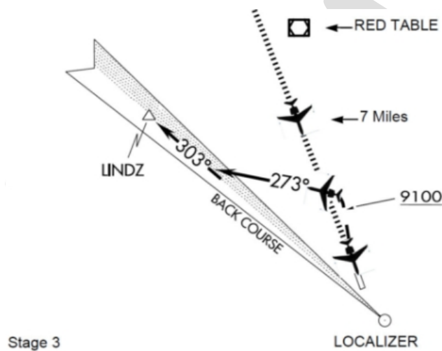
Figure 3 Opposite Direction Operation - Stage 3
