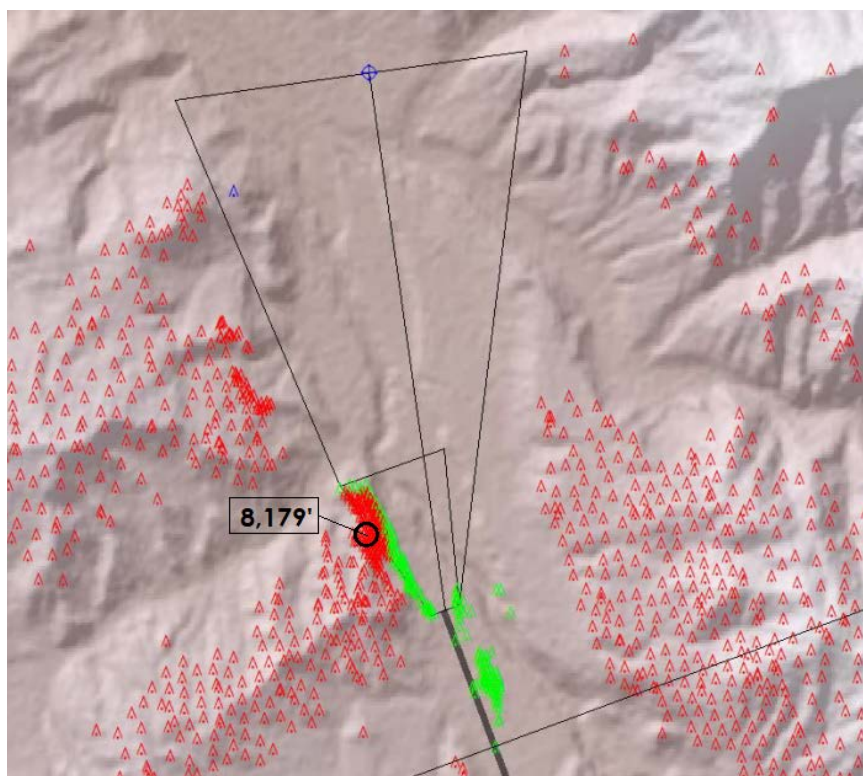
Figure 5 RWY 33 LINDZ 9 Low Close-In Obstacle Detection Area
