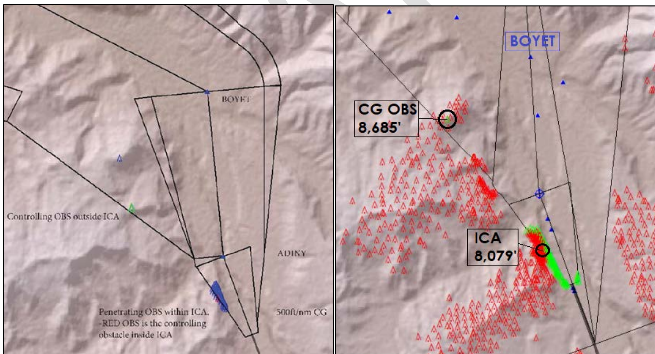
Figure 8 Low Close-In Obstacle Detection Areas Along PITKIN FOUR RNAV Departure
