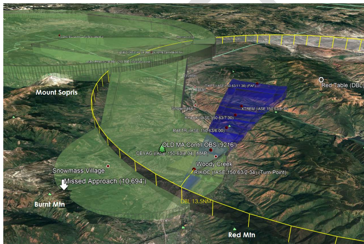
Figure 21 Depiction of Special LOC/DME Missed Approach Areas and DME Arc Limitation To Reduce Required Climb Gradient
