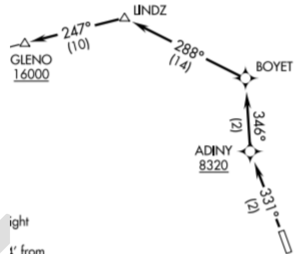
Figure 7 Current PITKIN FOUR RNAV Departure
