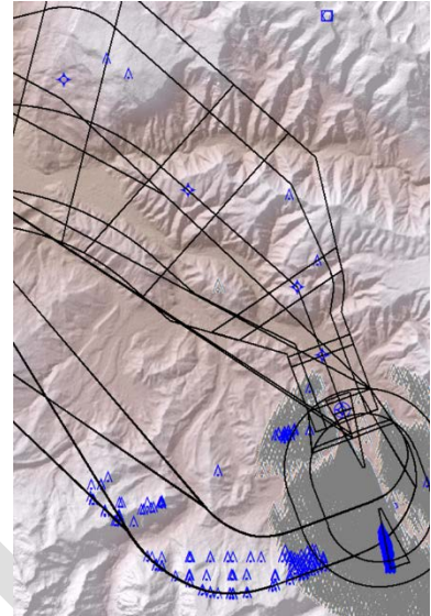
Figure 15 Expanded RNAV (GPS) -F OCS
