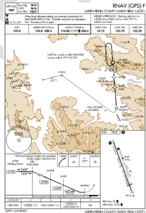
Figure 13 Current RNAV (GPS) -F Approach
