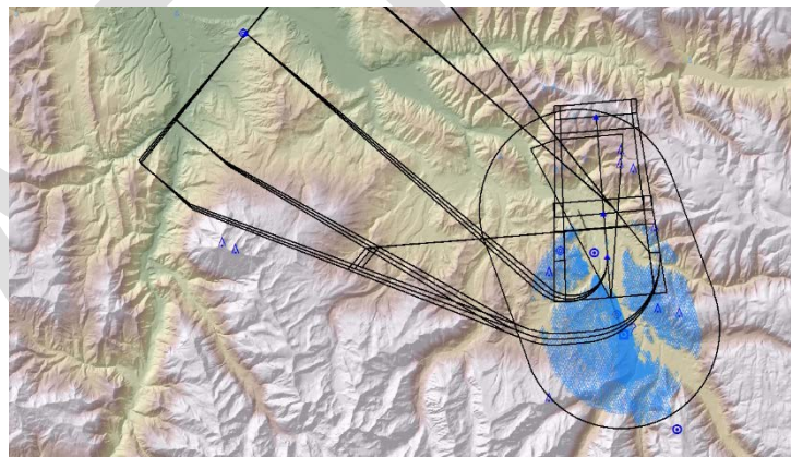
Figure 12 VOR-DME C OCS Areas
