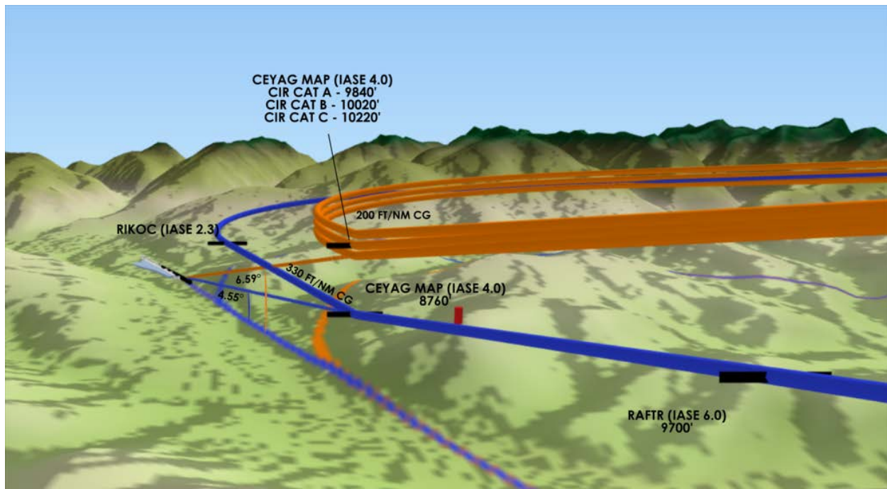
Figure 11 Standard LOC vs LOC Special Vertical Profile
