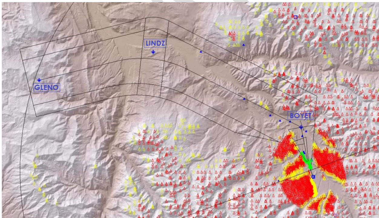
Figure 6 PITKIN FOUR Departure Obstacle Assessment Areas
